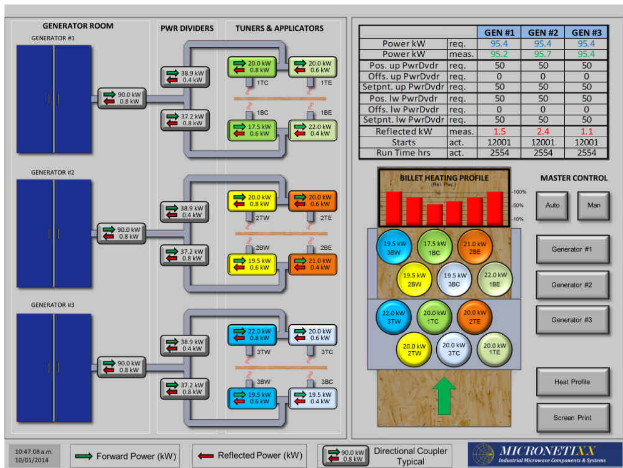
An Example of an HMI Screen for the Visuex™ Micronetixx LVL or MDF System Up-Grade
