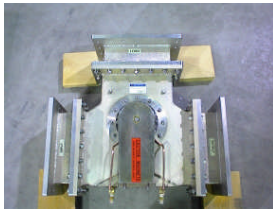
High-Power Circulators 75 kW and 100 kW
