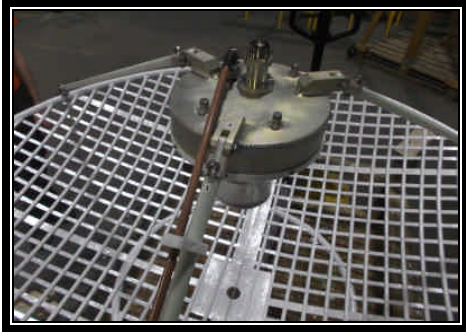
Special High-Gain, High-Power Circularly-Polarized L-Band Dish Antenna With its C-P Feed for the U. S. Military
