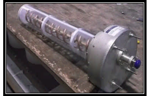
High-Power Circularly-Polarized 30° X 30° HPBW Antenna for the U. S. Air Force
